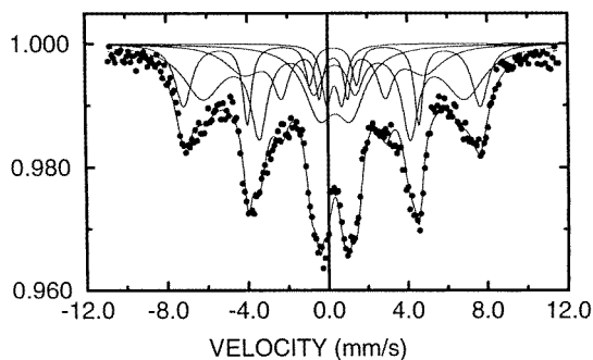
Figure 4. The Mössbauer spectrum recorded at 295 K for sample S29 with a magnetic field of 0.7 T.
